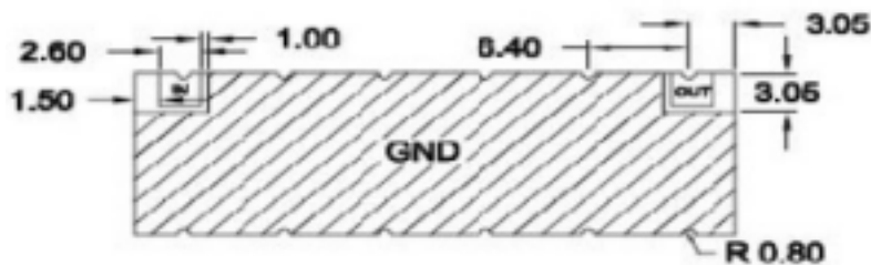
BOTTOM VIEW
